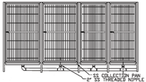
This plumbing can easily be joined together by your plumber. Collection pans in each run can be connected with PVC piping and plumbed to a central sewer line.
